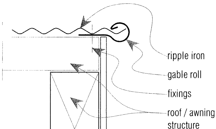
SECTION OF GABLE ROLL scale: 1 : 2 @ A4
