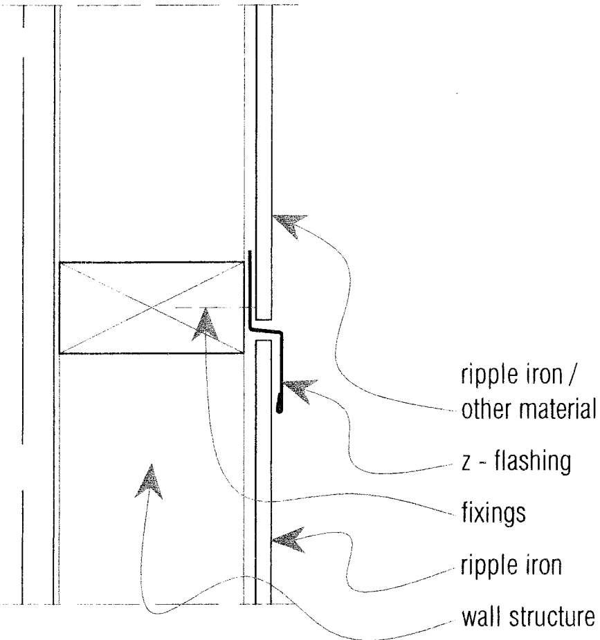
SECTION OF Z - FLASHING scale: 1 : 2 @ A4
